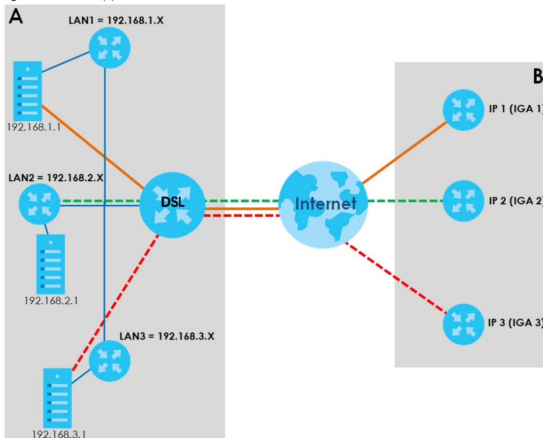
Figure 145 NAT Application With IP Alias
