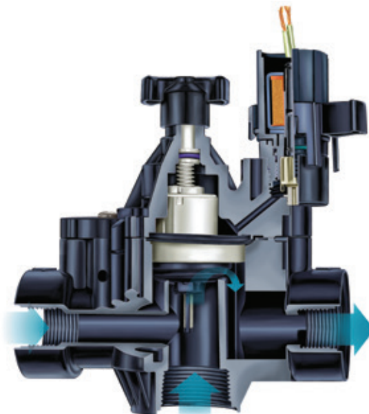
PGA Cutaway
