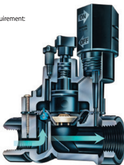
DVF Cutaway
