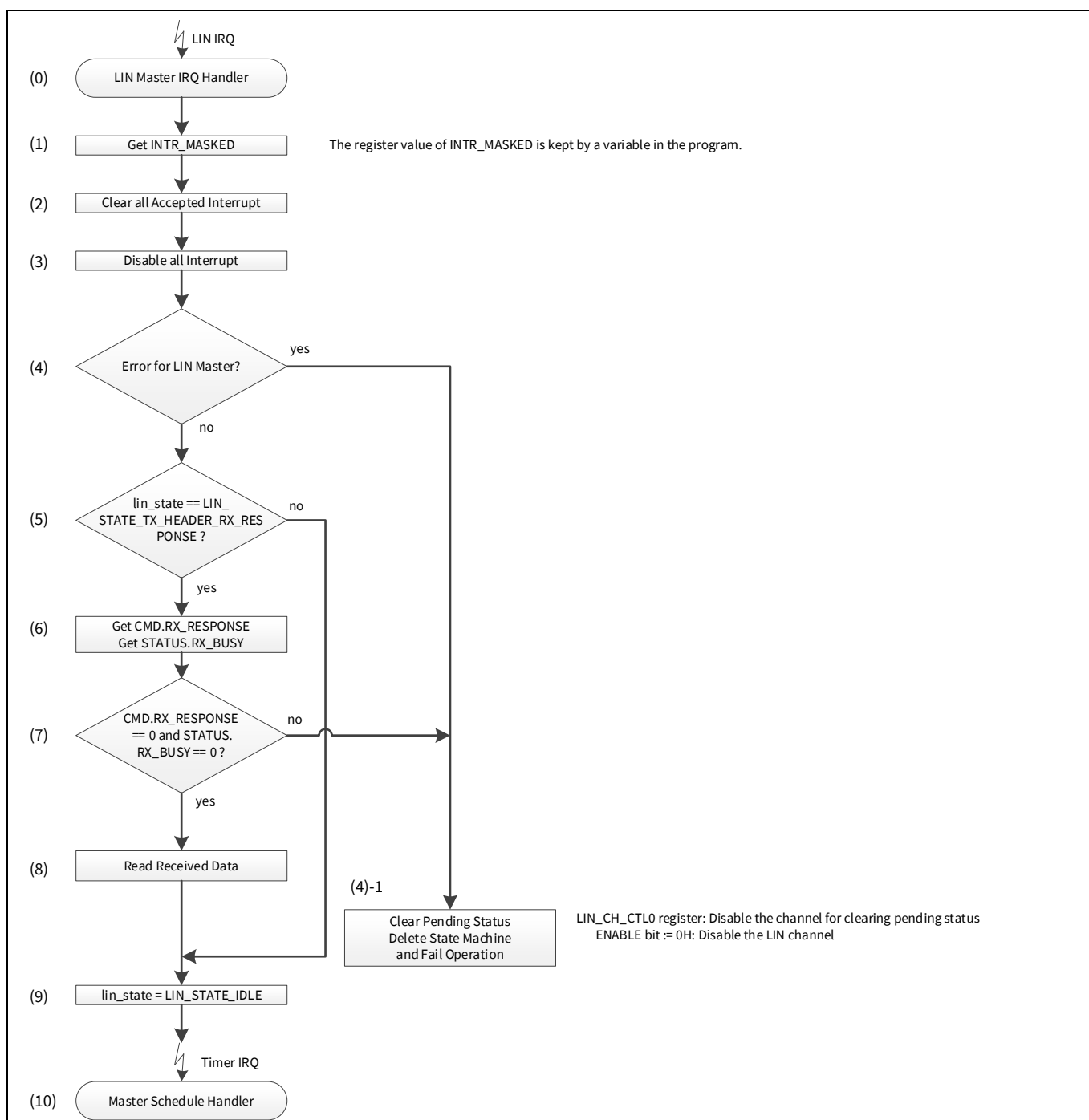
Figure 7 Example of LIN Master IRQ Handler
