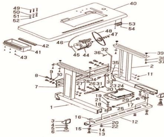
11. 机架、台板、电器分组件/Machine table electric components
