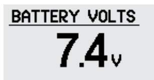
Example Screenshot
