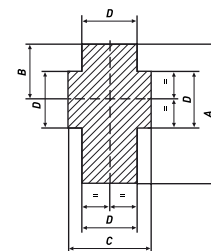
Figure 2 — Minimum dimensions of protected zones
