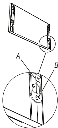
A. Shoulder Screw B. Locking Screw
