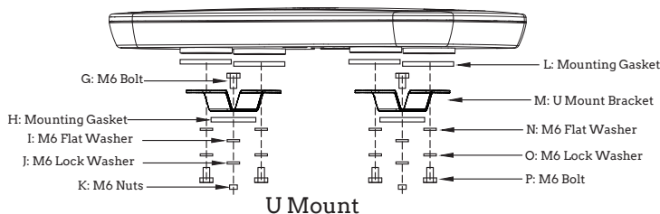
U Mount
