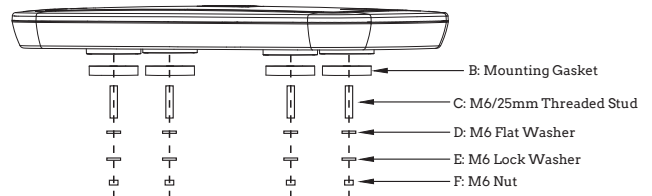
Bolt Mount
