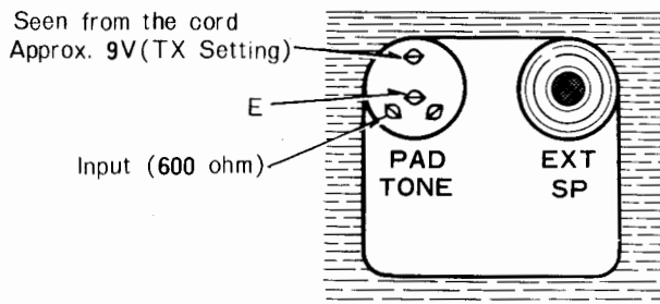
(a) TONE PAD Connector
