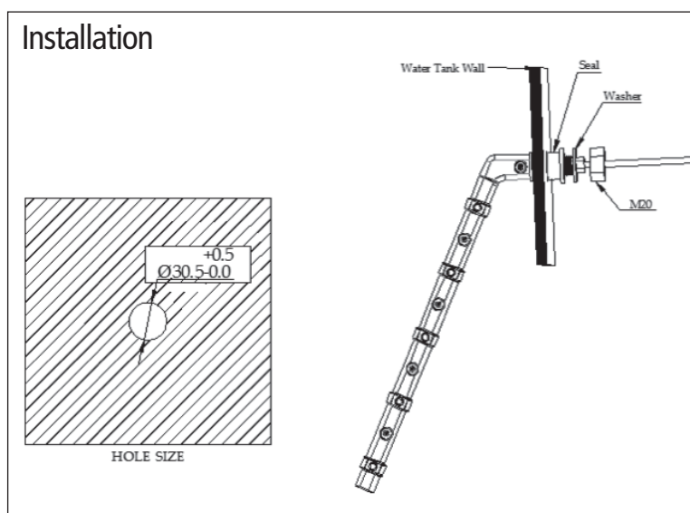
Figure 14 Installation of PMWS400
