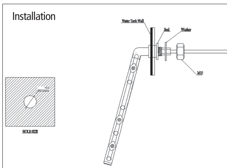
Figure 16 Installation of PMWS200
