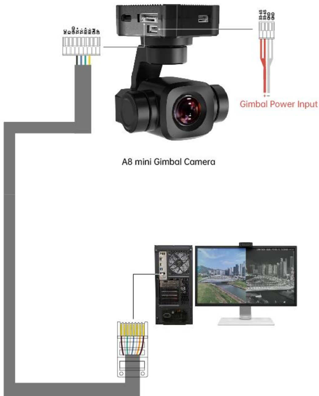
SIYI Gimbal Ethernet to RJ45 Cable (New)
