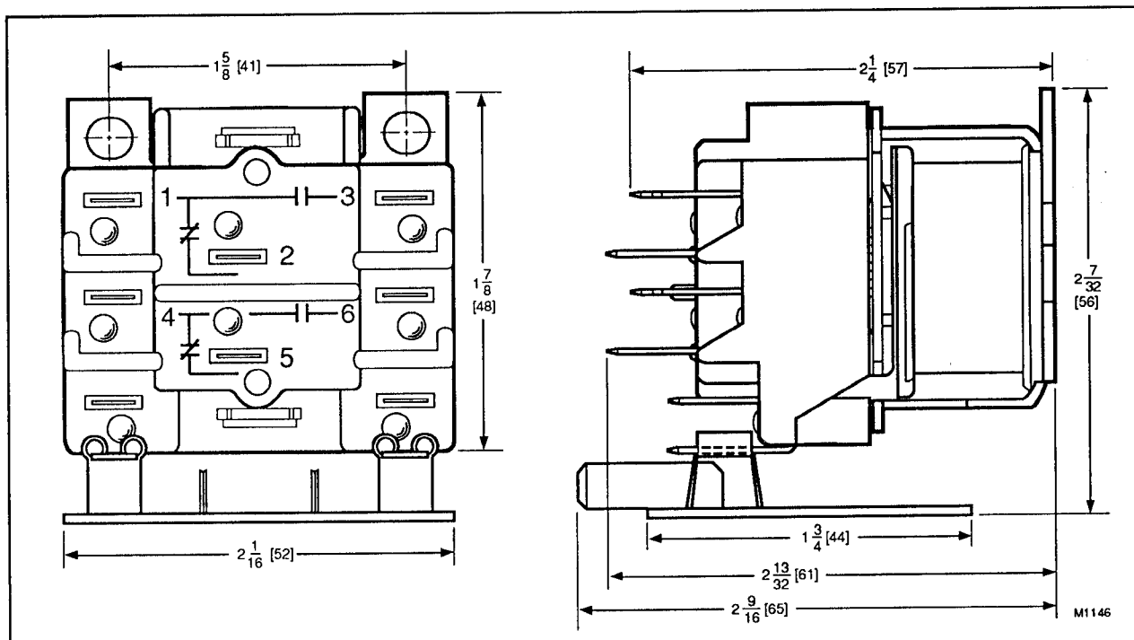
FIG. 2—APPROXIMATE DIMENSIONS OF ST82 IN in. [mm]. FOR APPLICATIONS REQUIRING EXACT ENGINEERING DIMENSIONS, CONTACT YOUR HONEYWELL SALES REPRESENTATIVE.
