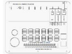
Typical Load Center Panel w/120V Main Breaker (Appearance and configuration may vary by model)
