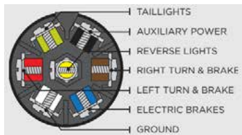
View from Trailer Wire Entry Side
