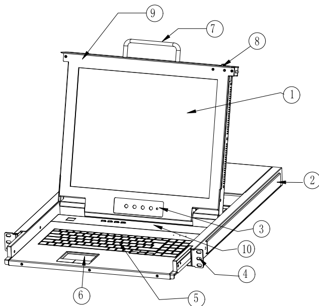
Figure 1-1 front view
