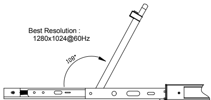
Figure 2-2 rotate angle of the console
