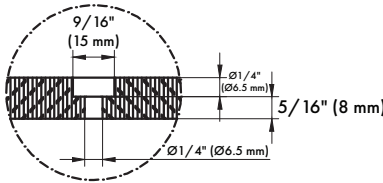
SECTION C
