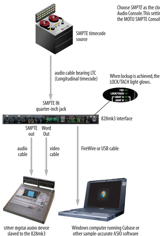
Figure 4-17: Connections for synchronizing the 828mk3 directly to SMPTE timecode.
