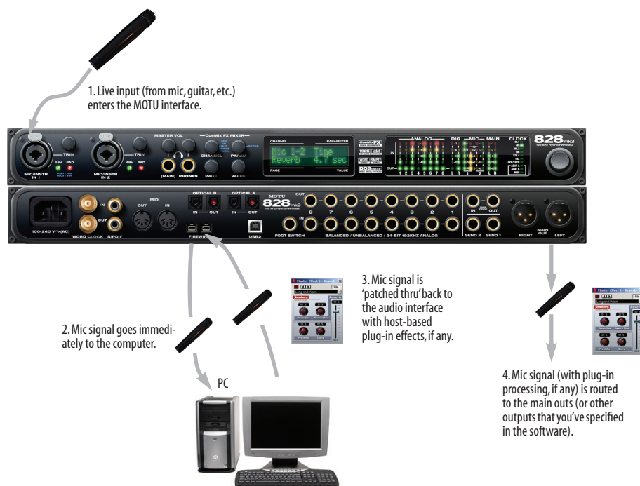
Figure 8-1: There are two ways to monitor live audio inputs with an 828mk3: 1) through the computer or 2) via CueMix FX hardware monitoring. This diagram shows method 1 (through the computer). When using this method, use your host software's buffer setting to reduce the slight delay you hear when monitoring the live input, but don't lower it too much, or your computer might get sluggish.
