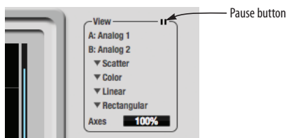
Figure 9-50: View controls
