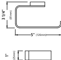
Model #: KEA-19929 Toilet Paper Holder Dimensions: 5" x 3 1/4" x 1"
