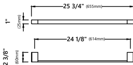
Model #: KEA-19937 Towel Bar Dimensions: 25 3/4" x 2 3/8" x 1"
