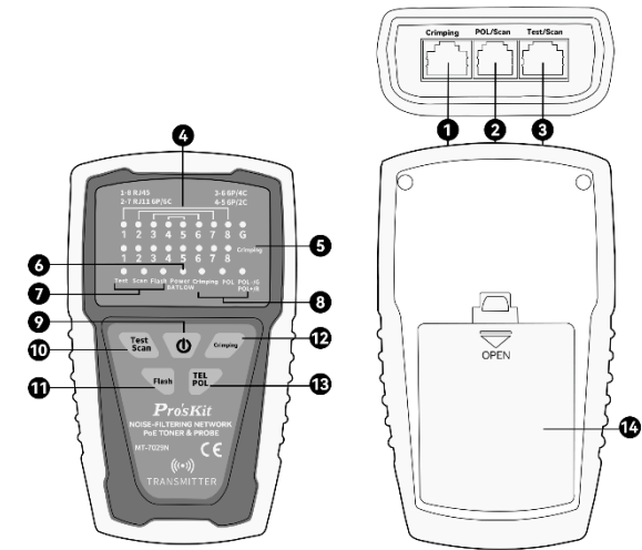
Figure1. MT-7029N Transmitter Diagram
