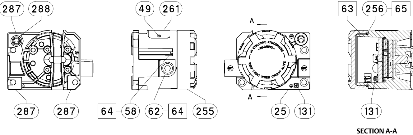
Figure 7-5. FIELDVUE DVC6215 Remote Feedback Assembly
