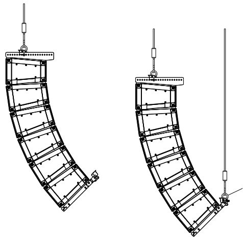
X12TC-GRID WITH PULL-BACK TO VENUE
