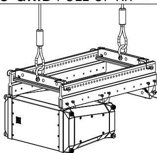
X12TC-GRID PULL-UP KIT
