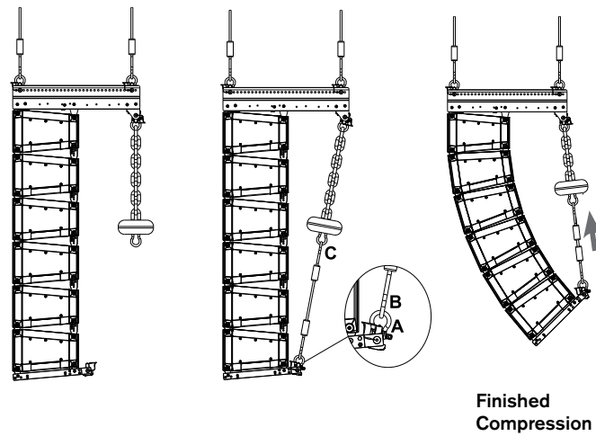
X12TE-GRID X12PU-BGK TO PULL-UP TO GRID
