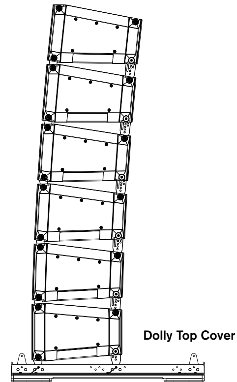
Dolly Top ground-stacking
