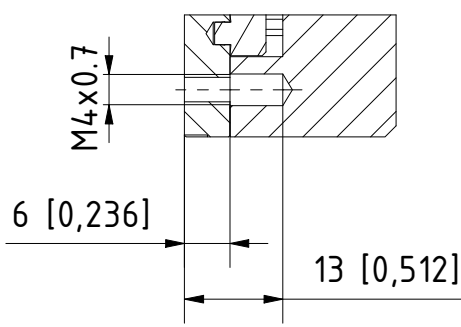
A-A View for bolt hole
