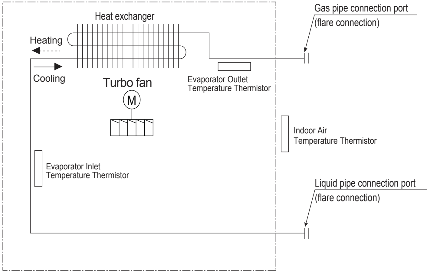
Figure 19: LCN097, 127HV4 Refrigerant Flow Diagram.
