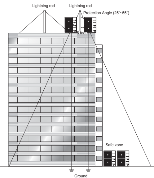
Figure 36: Lightening Protection Diagram.
