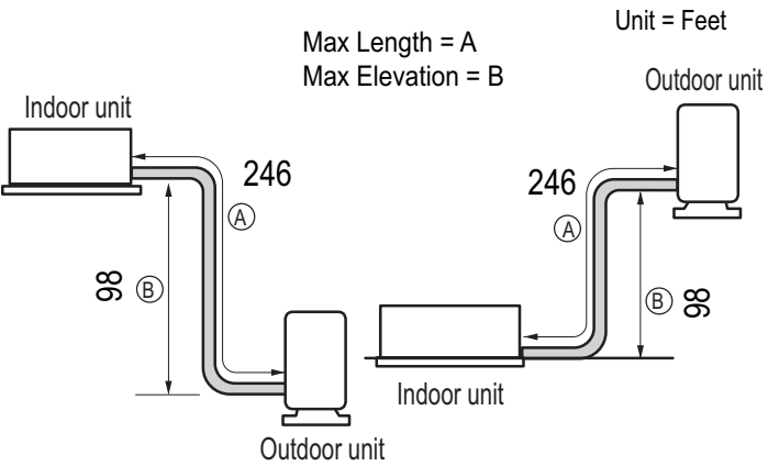
Figure 46: Typical LC347HV and LC427HV System Layout.
