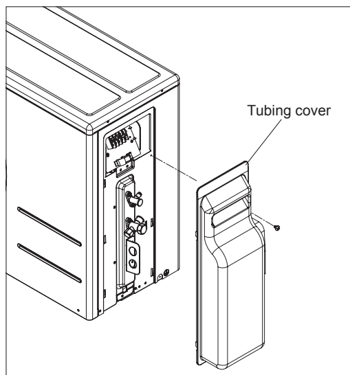
Figure 55: Removing the Refrigerant Piping Connection Cover (LUU097HV, LUU127HV).
