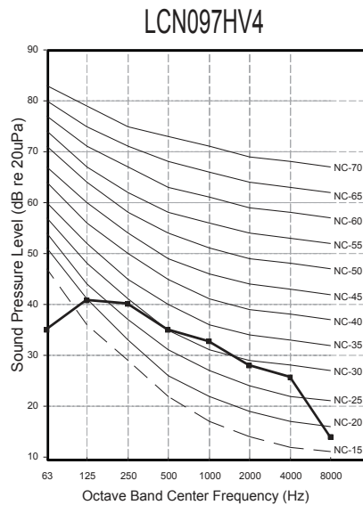
Figure 11: Four-Way Ceiling Cassette Indoor Unit Sound Pressure Level Diagrams.
