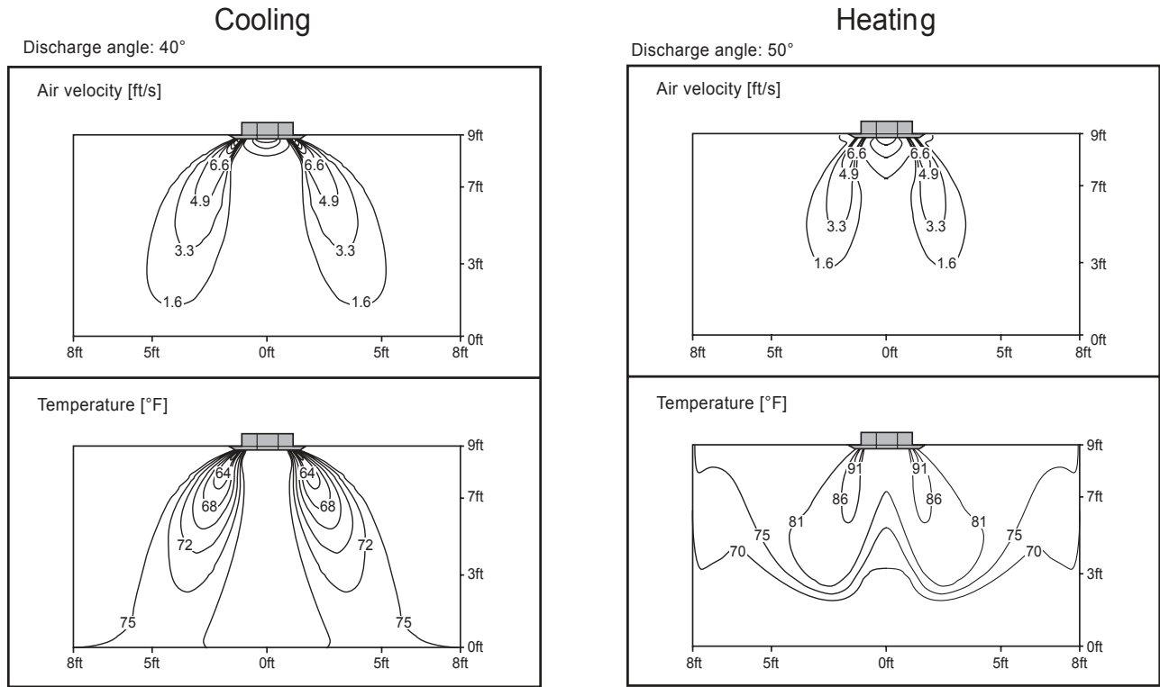
Figure 12: LCN097HV4 Air Velocity and Temperature Distribution Charts.
