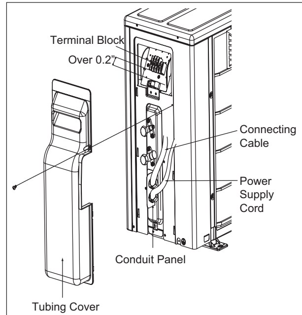
Figure 63: LUU097, 127HV Outdoor Unit Terminal Block Location.
