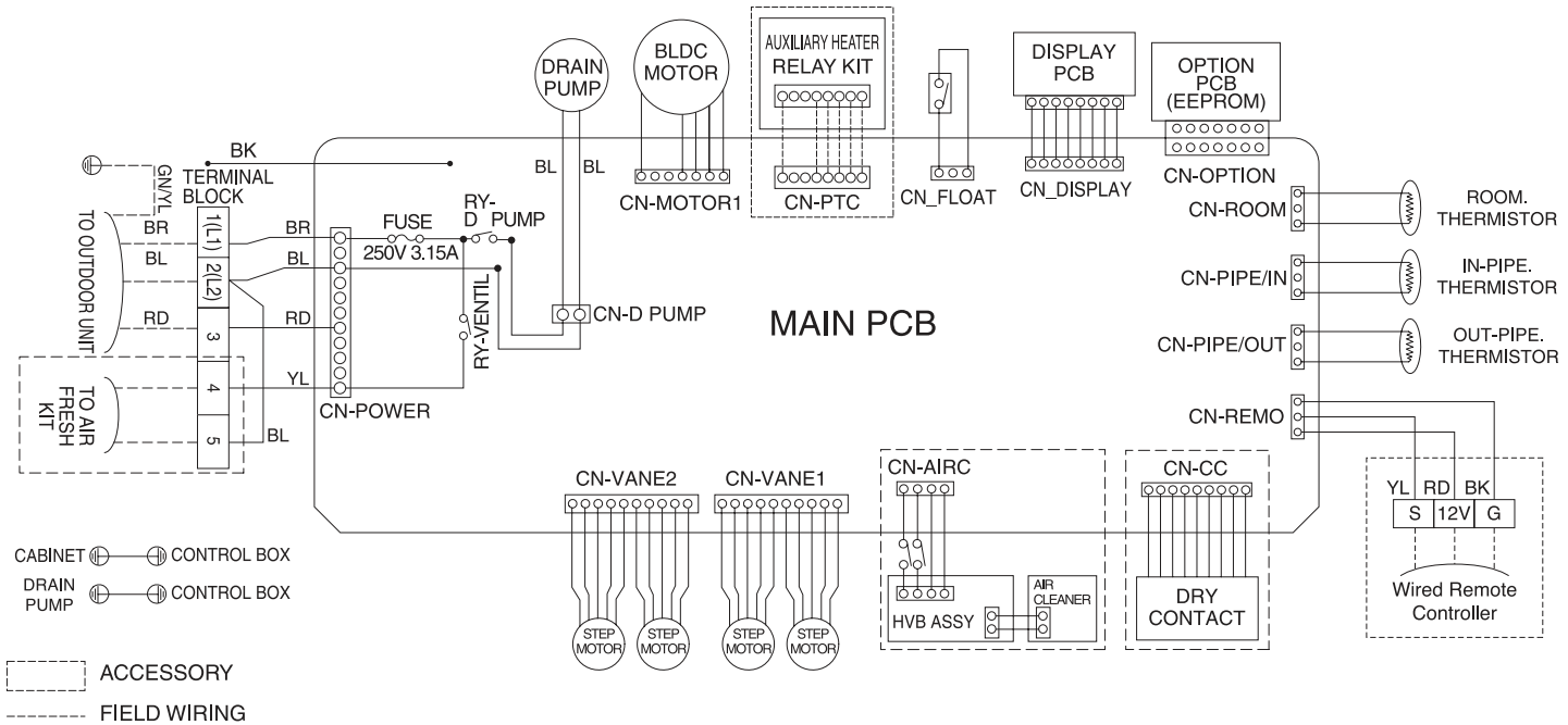
Figure 25: Four-Way Ceiling Cassette LCN097, 127HV4 Indoor Unit Wiring Diagram.
