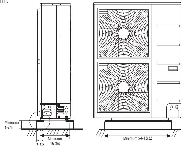
Figure 41: Platform Mounting.
