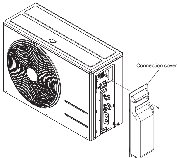
Figure 56: Removing the Refrigerant Piping Connection Cover (LUU187HV, LUU247HV).
