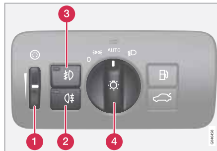
Overview, light switches with AUTO function
