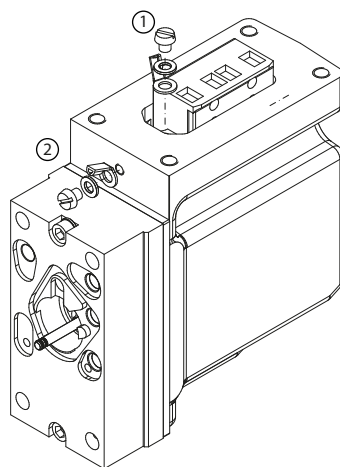
Connector terminal
