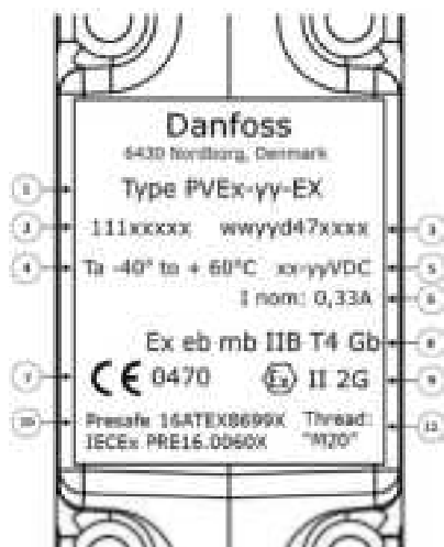
Nameplate for PVE-EX Ex eb mb version
