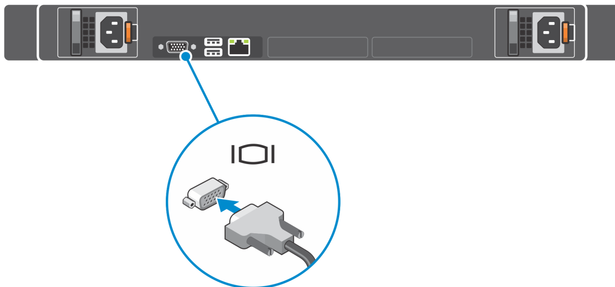
Figure 8. Display port
