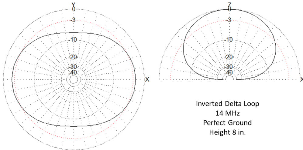
Figure 4. Inverted Delta Loop Far Field Plot.
