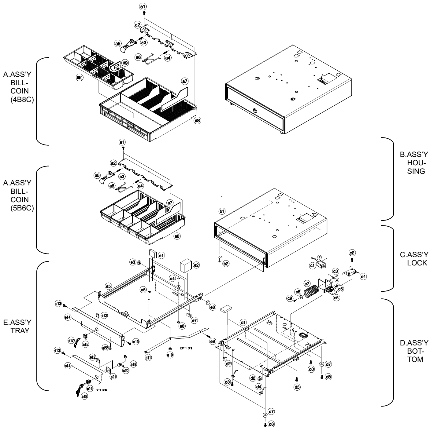
Figure 6-9 ASS'Y-DRAWER (G-DRAWER:4B8C,5B6C)
