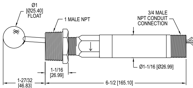
Round stainless steel float
