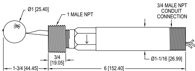
Polypropylene float
