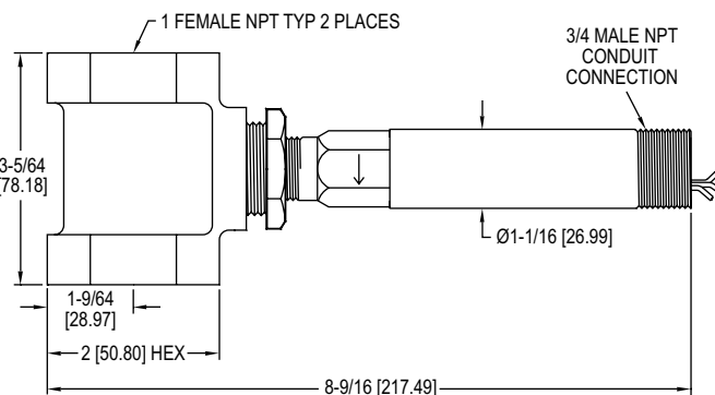
With external chamber (tee)
