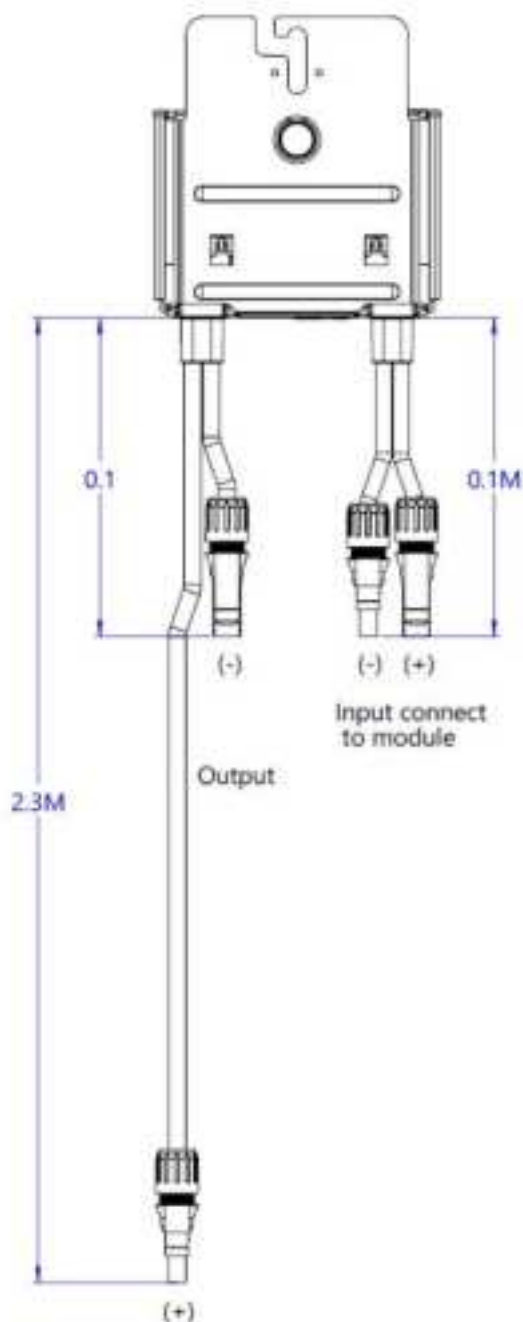
Figure 2: Comparing the S-Series and P-Series Power Optimizer Input and Output Wires and Dimensions.
