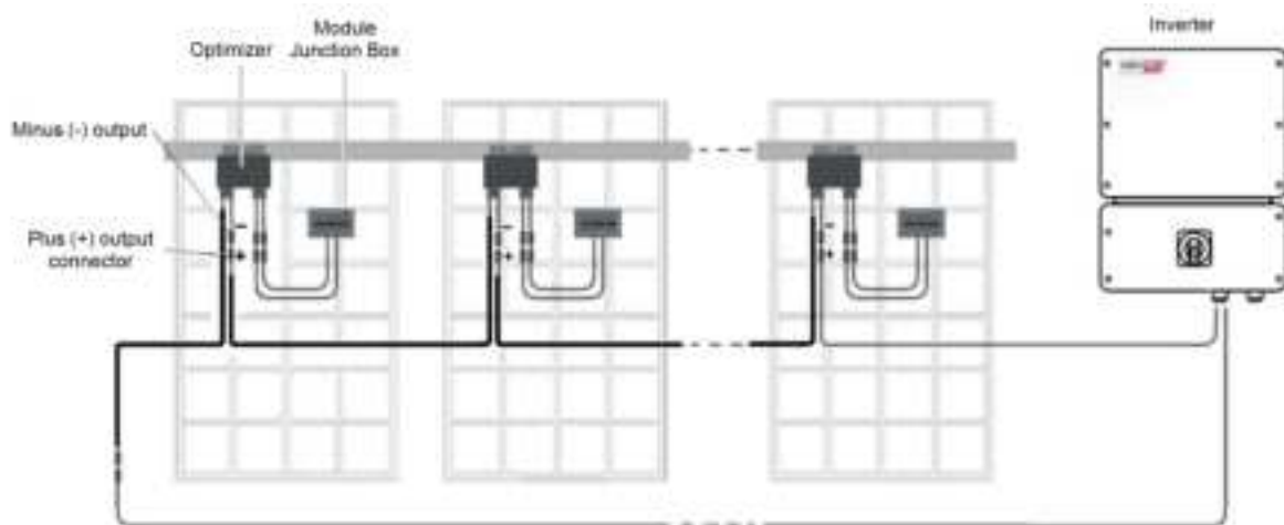
Figure 3: S-Series Input and Output Wire Connection Schematic.
