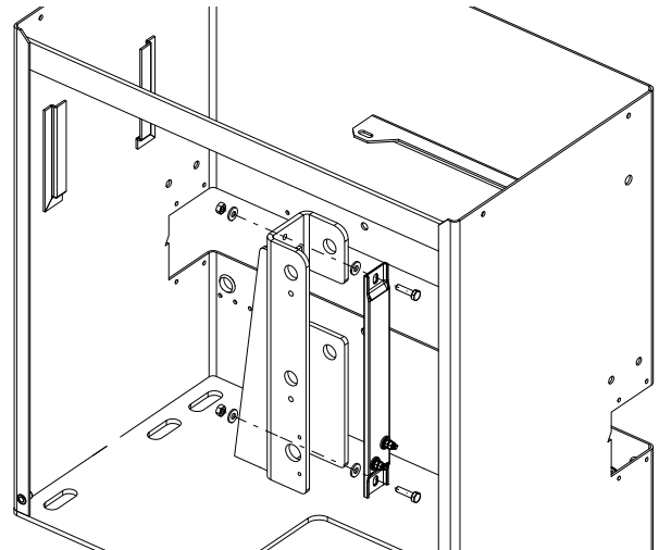
Figure 7. Install Heater Strip
