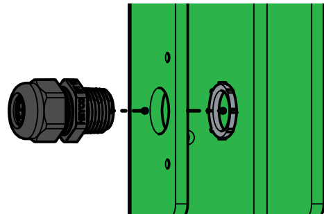
Figure 8. Strain Relief
