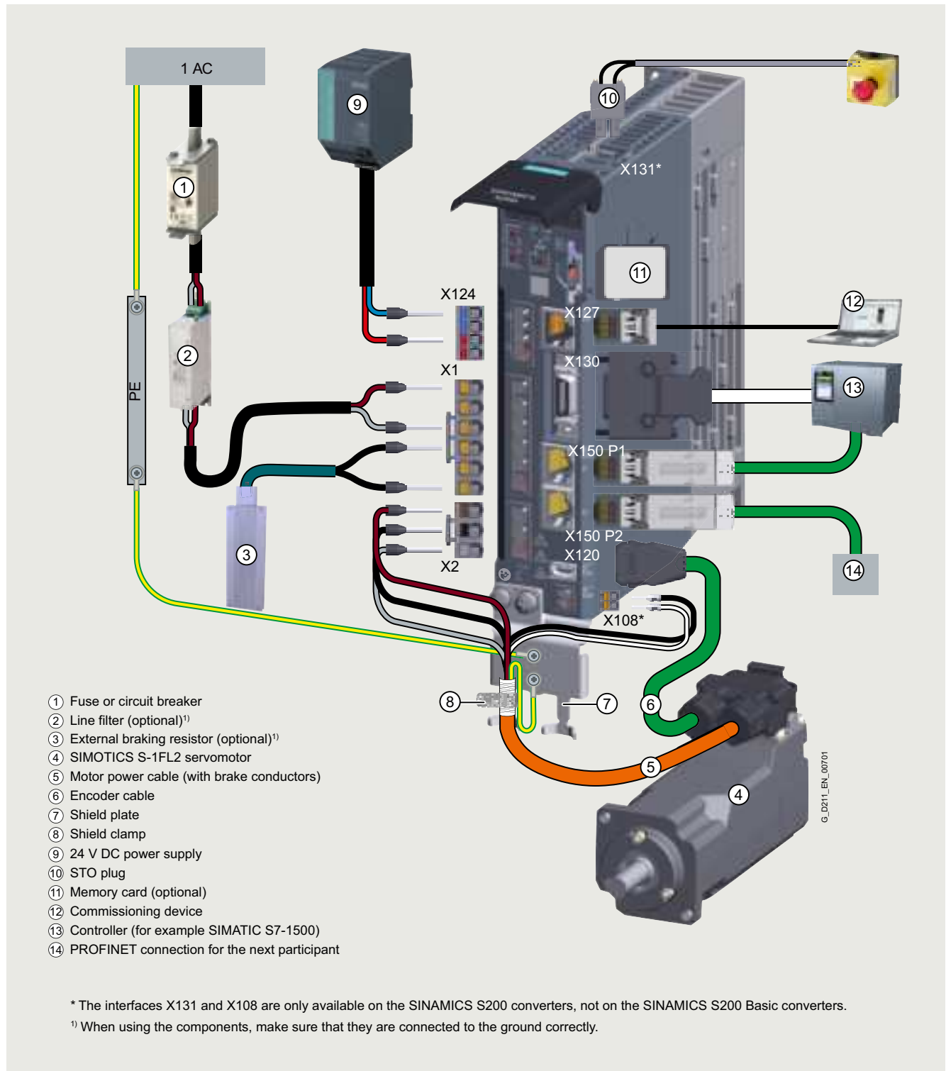
System connection overview SINAMICS S200 servo drive system, PROFINET version, 1 AC
