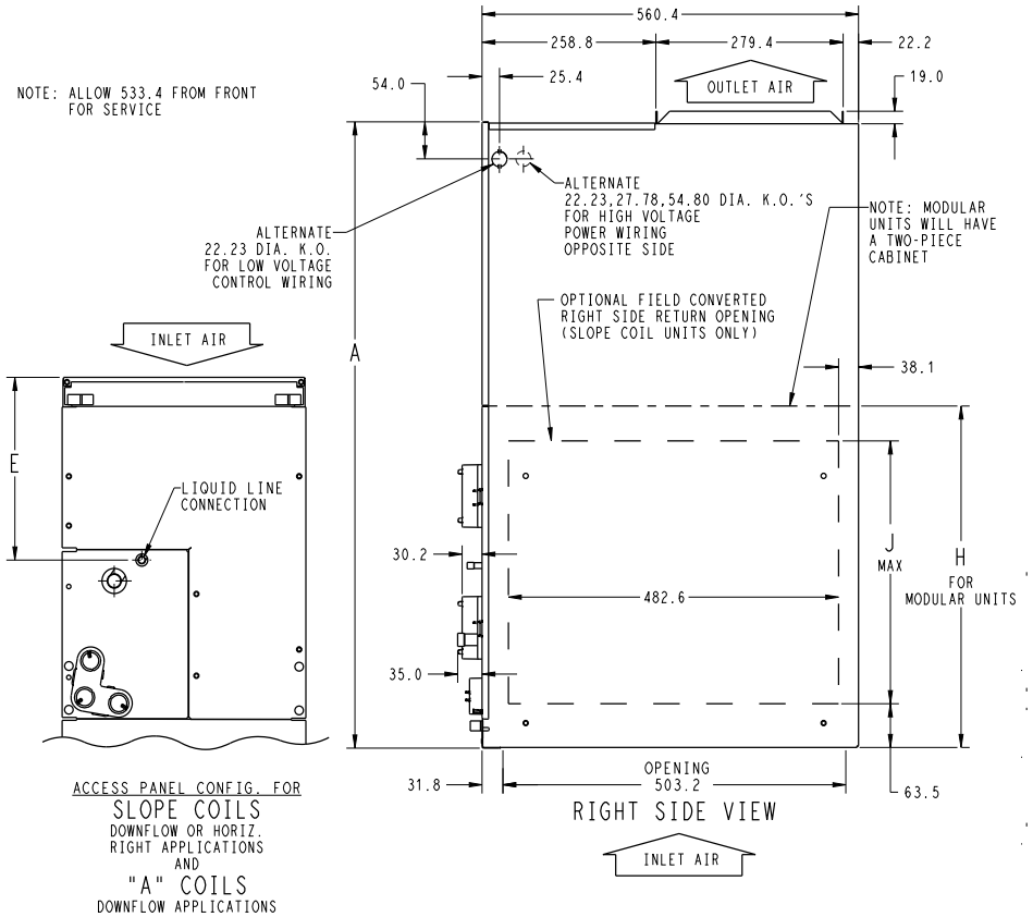
Fig. 3 – Dimensions, sheet 3
