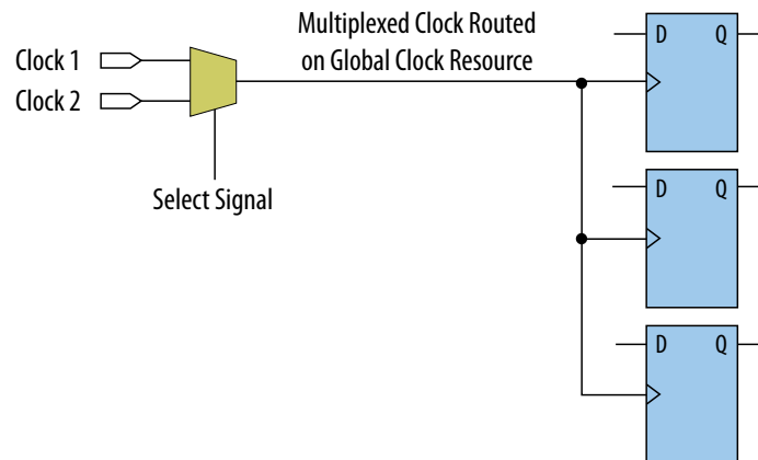
Figure 10. Multiplexing Logic and Clock Sources
