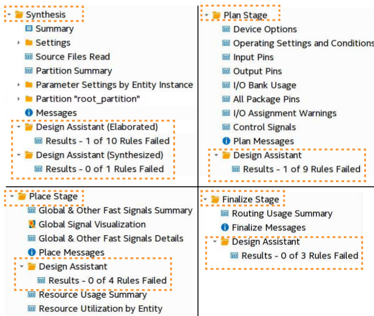
Figure 24. Example Design Assistant Results in Compilation Reports
