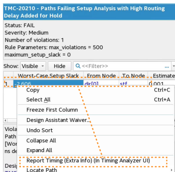
Figure 32. Cross Probing from Design Assistant Rule TMC-20210 Violations to Timing Analyzer
