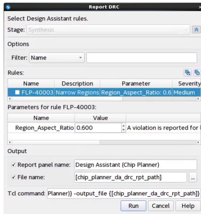
Figure 27. Report DRC Dialog Box in Chip Planner
