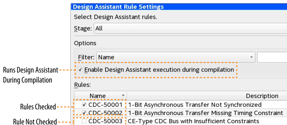
Figure 23. Design Assistant Rule Settings
