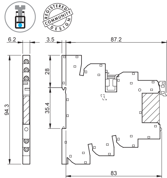
Types 39.30/39.30.3 39.31/39.31.3 Bornes à cage
