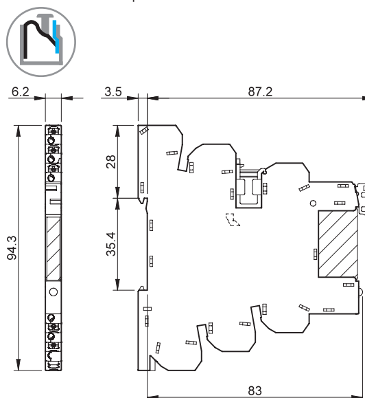
Types 39.60/39.60.3 39.61/39.61.3 Bornes automatiques
