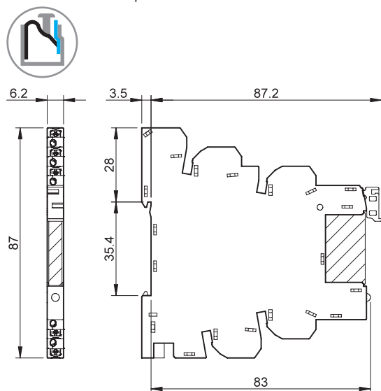
Types 39.00/39.01 39.50/39.51 Bornes automatiques
