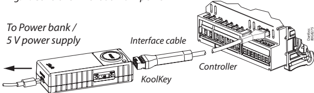
Fig. 4: Controller without main power
