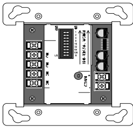
4090-9010 8 A IDNet Relay IAM Package
