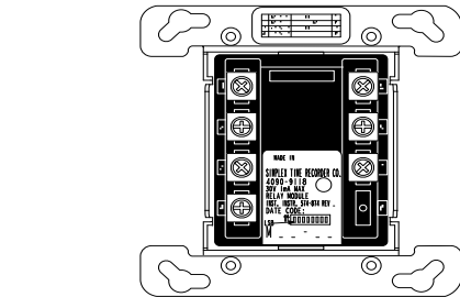
4090-9118 Relay IAM with T-Sense Input
