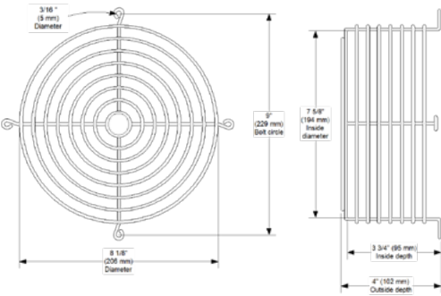
2098-9715 Wire Guard
