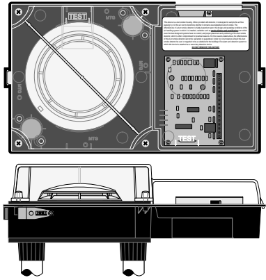
Duct Sensor Housing, Front and Bottom View
