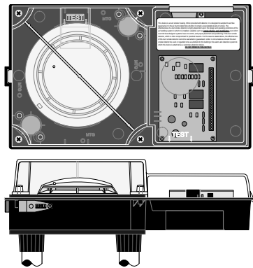
Duct Detector Housing, Front and Bottom View
