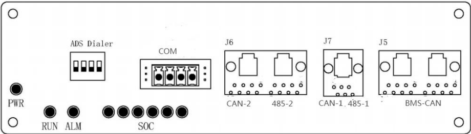
Fig. 5-2 Peration Panel
