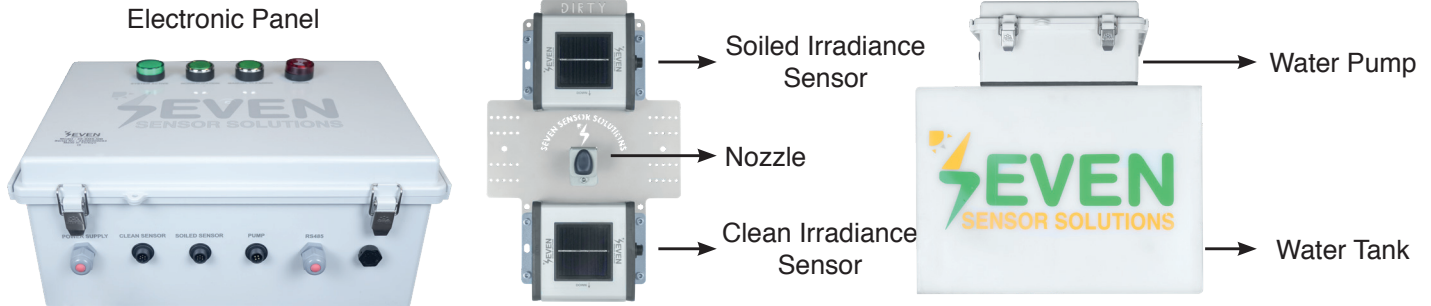
Figure 1 – Components of the Automatic Soiling Sensor
