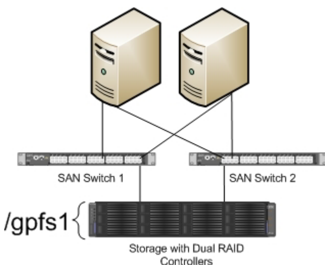
Figure 6. An example of a highly available SAN configuration for a GPFS file system
