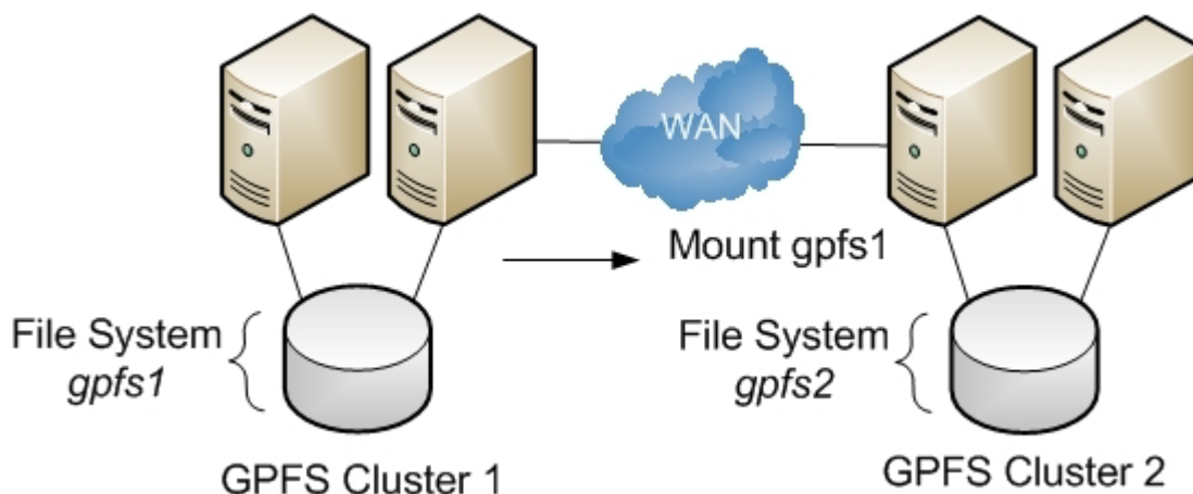
Figure 2. A multicluster configuration
