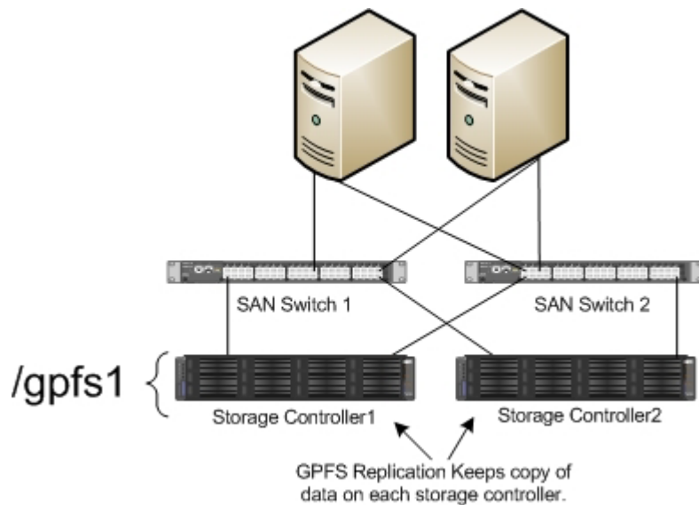
Figure 7. Configuration using GPFS replication for improved availability
