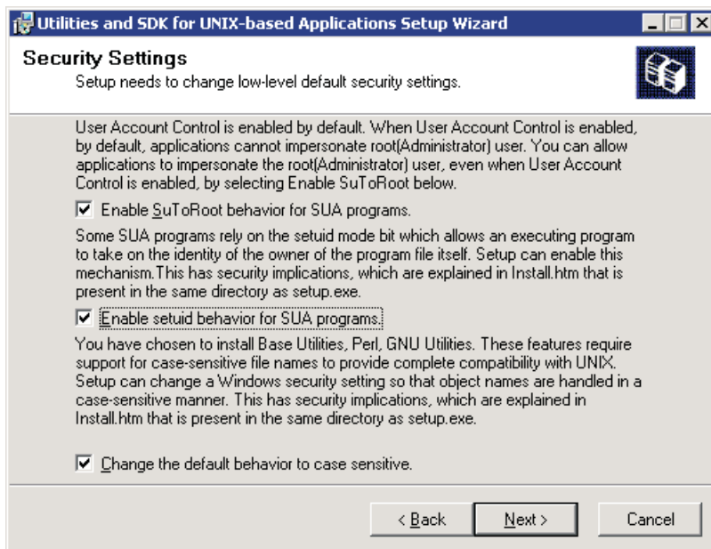
Figure 9. Utilities and SDK for UNIX-based Applications Setup Wizard - Security Settings
