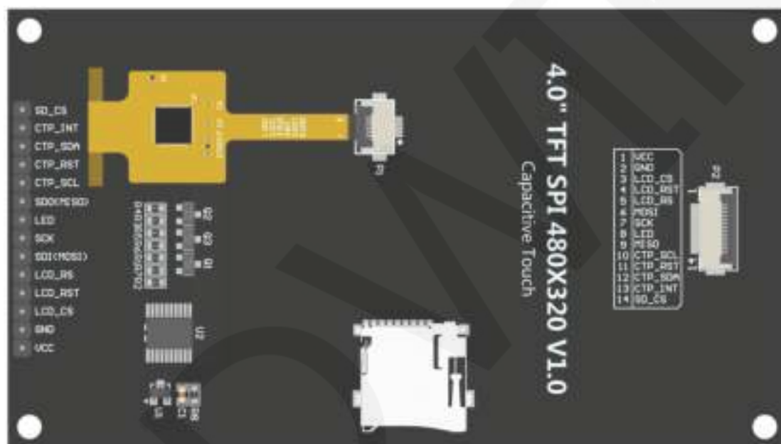
Picture1. Module Back Pins
