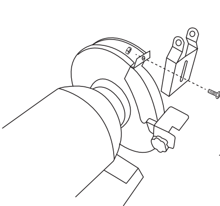
Installing Spark Guards
