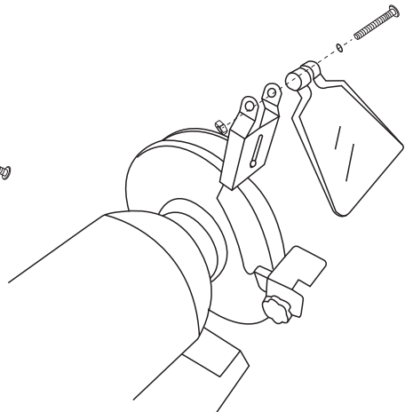
Installing Eye Shield to Grinder
