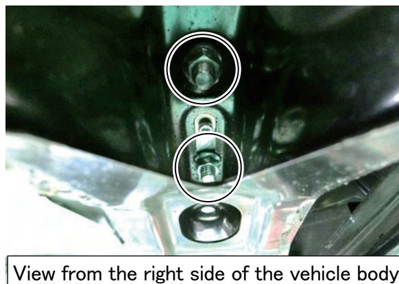
Fig. 5 M10Bolt, Flange nut mounting position
