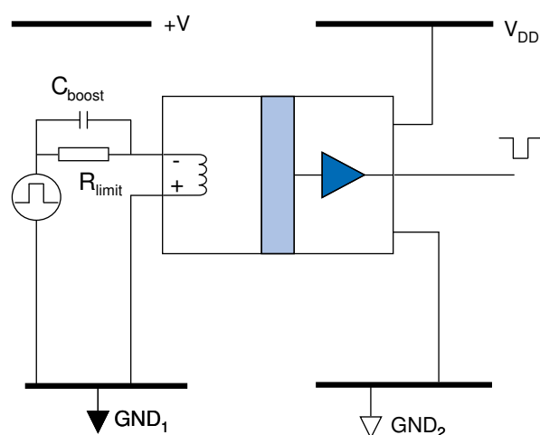
Inverting Configuration
