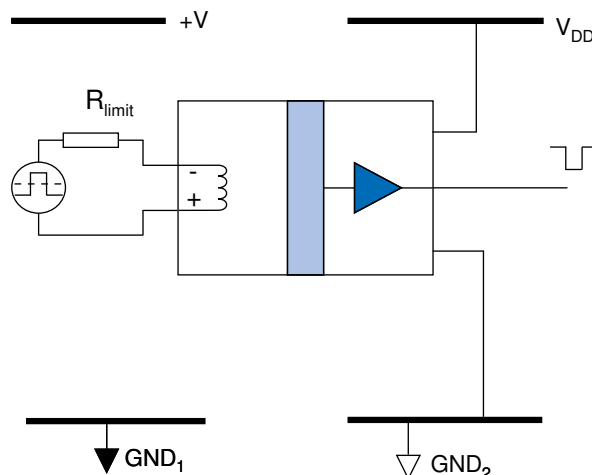
Differential Configuration
