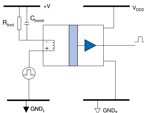
Non-inverting Configuration
