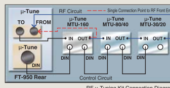
RF μ-Tuning Kit Connection Diagram
