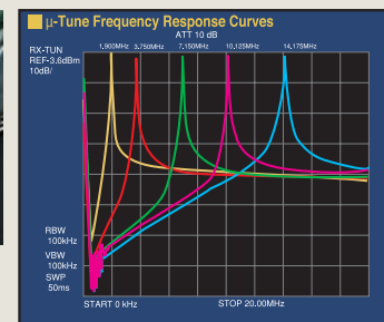
10 dB/Div • 2 MHz/Div
