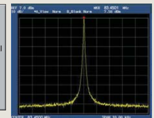
Carrier-to-Noise (C/N) Characteristics
