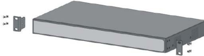
Figure 3-1 Install bracket
