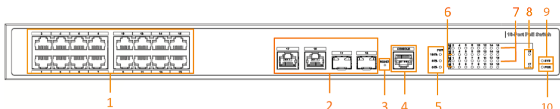
Figure 2-1 Front panel
