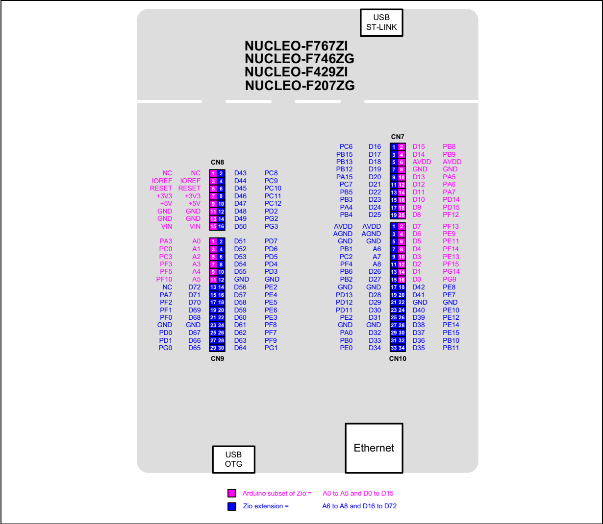
Figure 11. NUCLEO-F767ZI, NUCLEO-F746ZG, NUCLEO-F429ZI and NUCLEO-F207ZG
