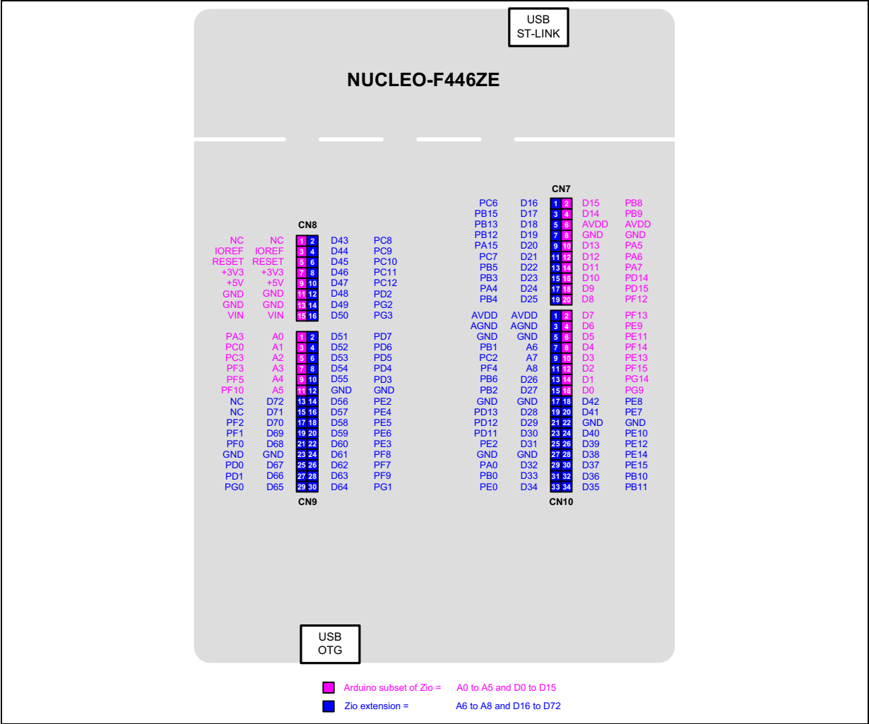
Figure 14. NUCLEO-F446ZE
