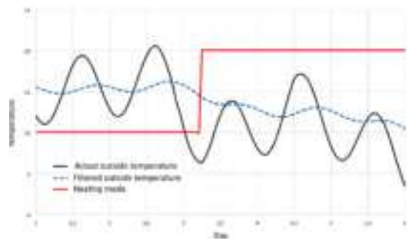
Fig. 04-1 Heating mode started by filtered outside temperature
