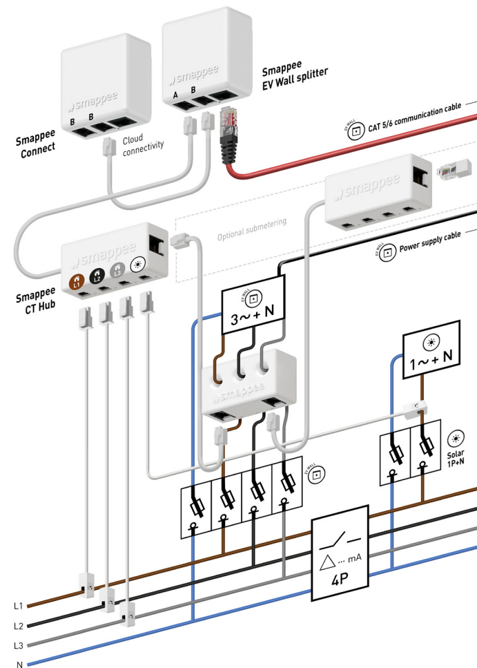
EV Wall three phase connection diagram.
