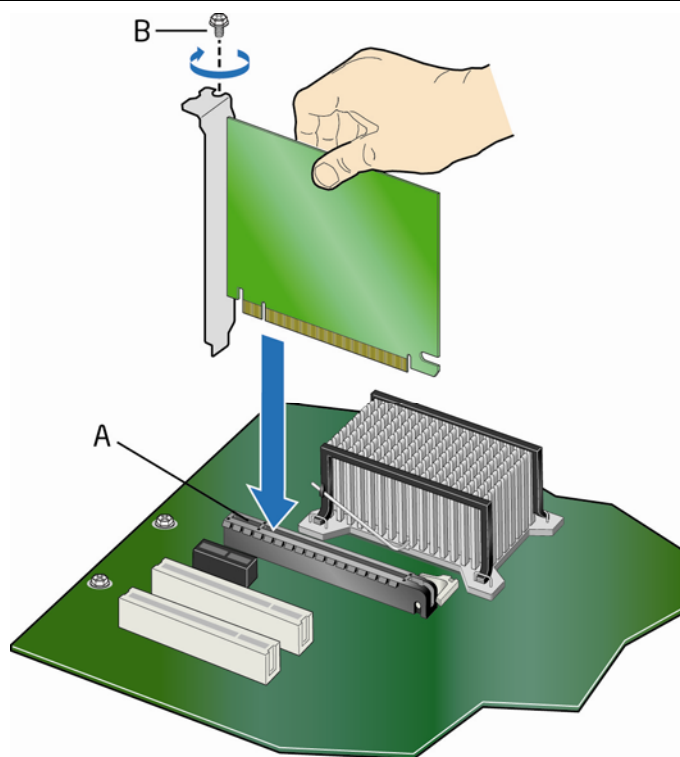
Figure 16. Installing a PCI Express x16 Card
