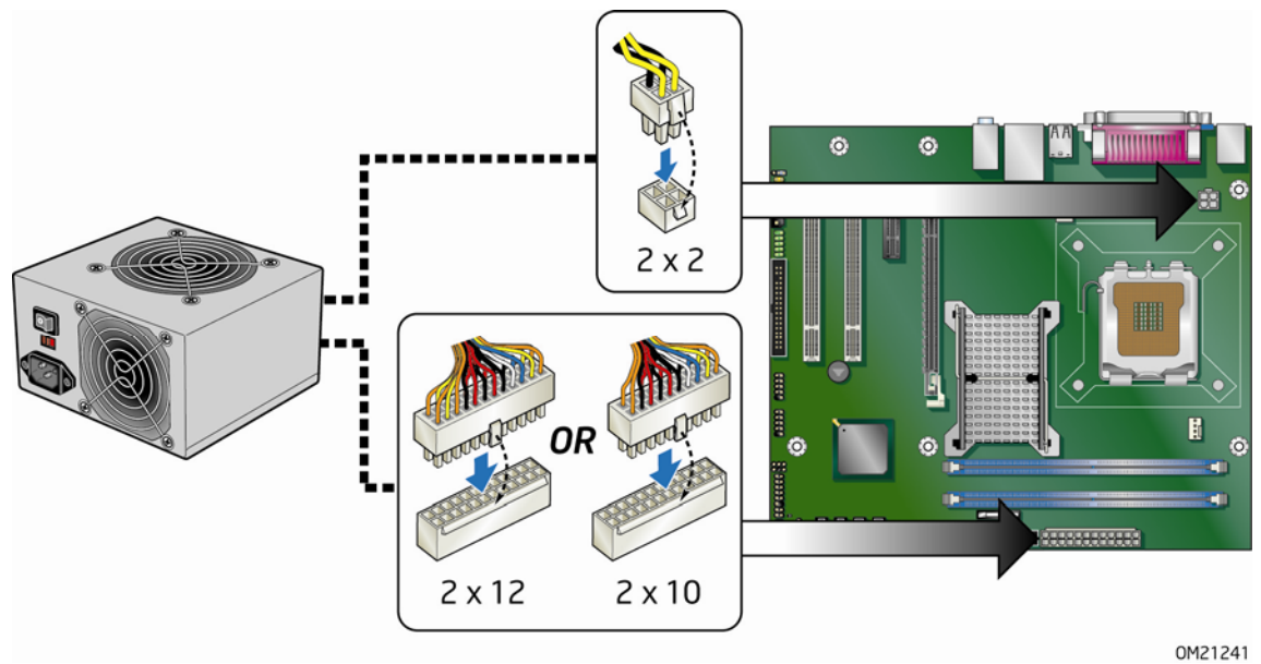
Figure 24. Connecting Power Supply Cables
