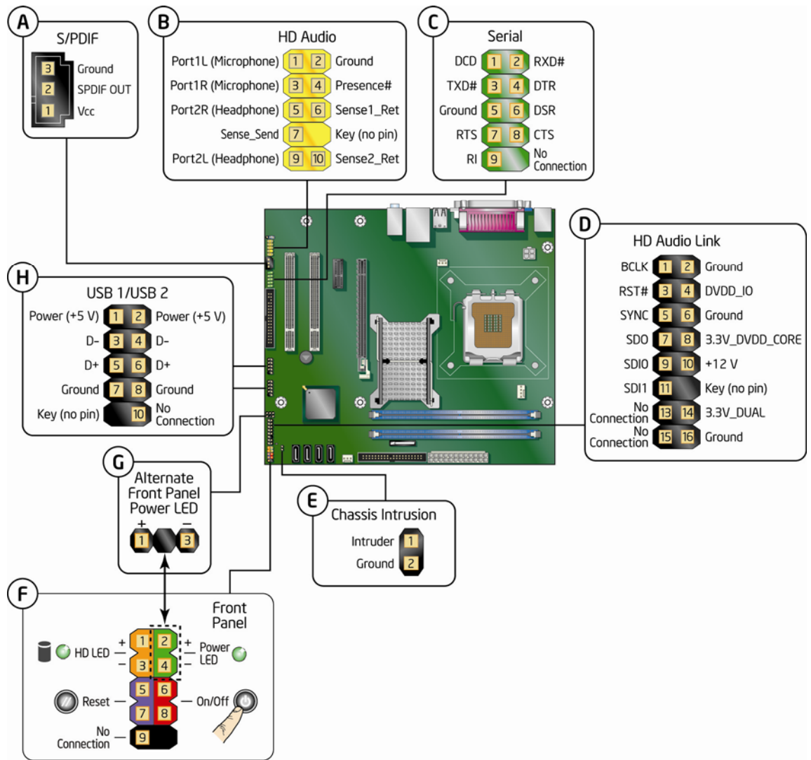
Figure 21. Internal Headers and Connectors
