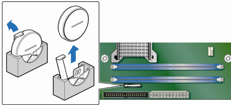
Figure 26. Removing the Battery
