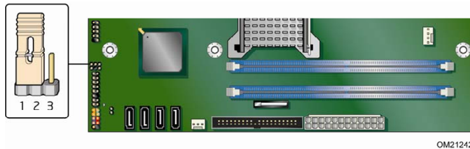
Figure 25. Location of the BIOS Configuration Jumper Block
