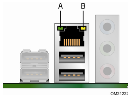
Figure 2. LAN Connector LEDs
