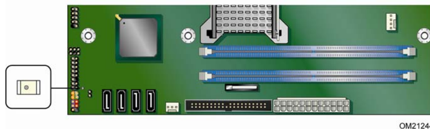
Figure 3. Location of the Standby Power Indicator
