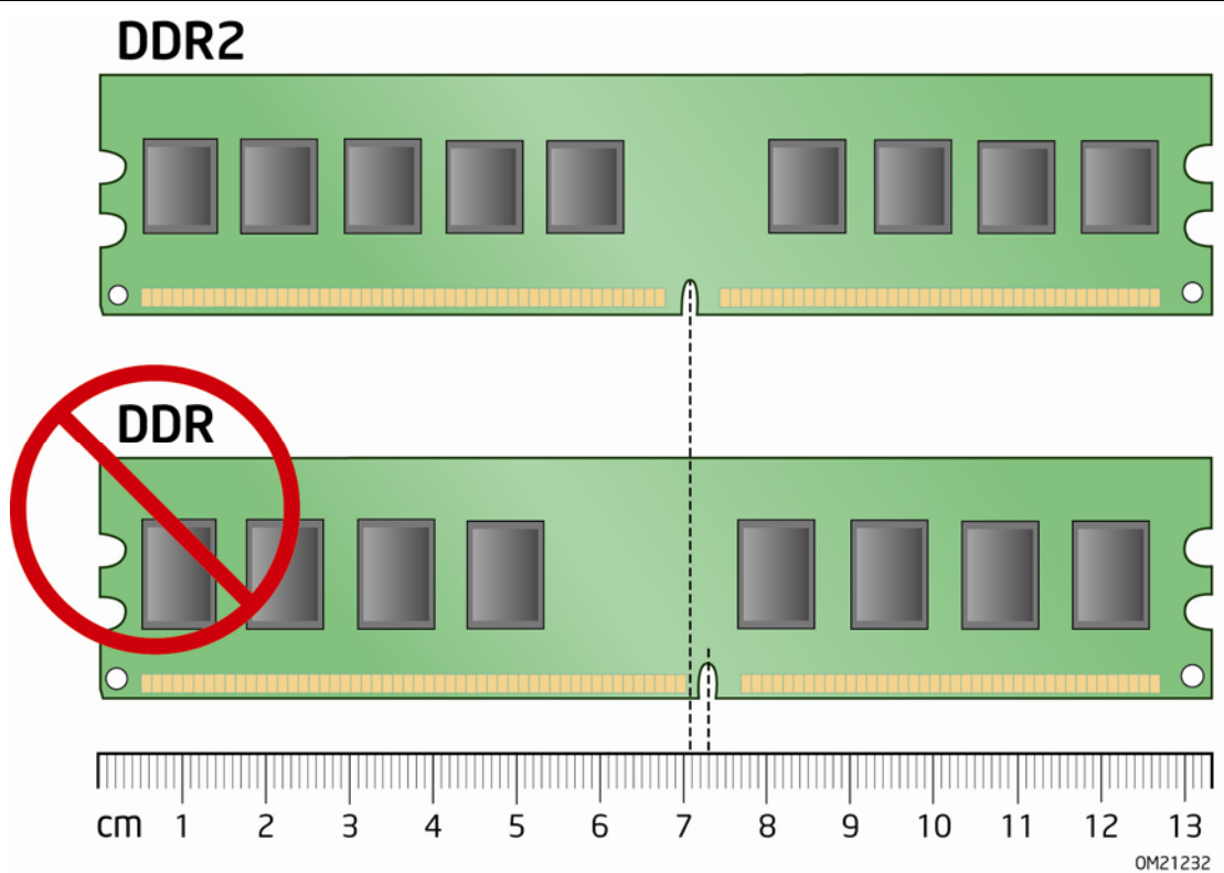
Figure 14. Use DDR2 DIMMs
