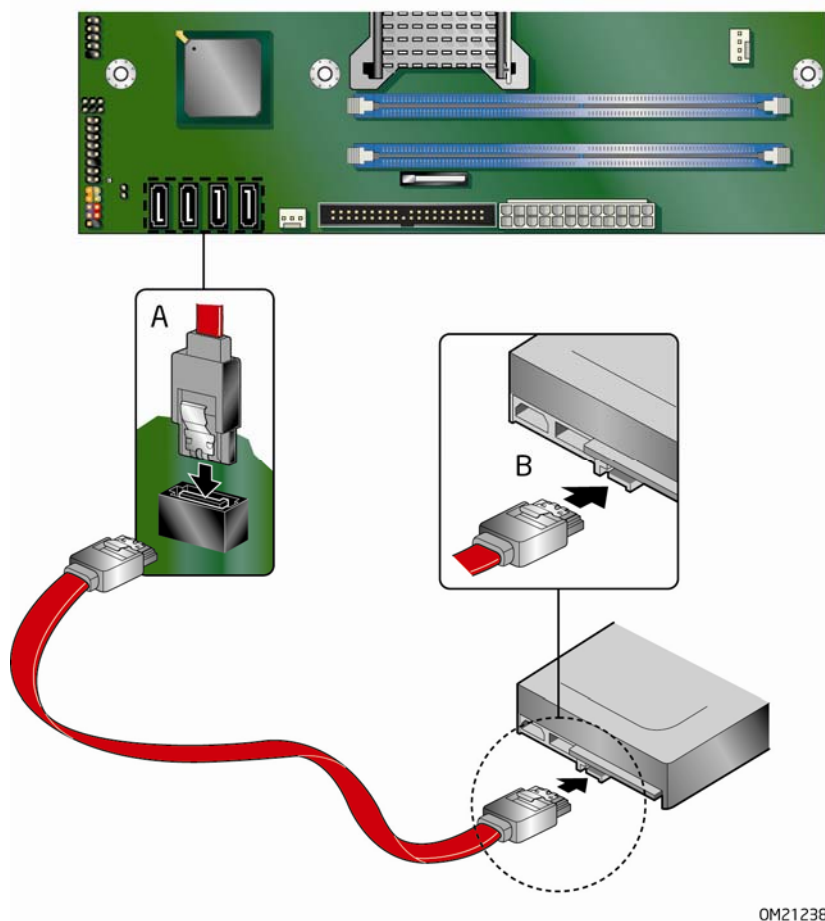
Figure 20. Connecting a Serial ATA Cable
