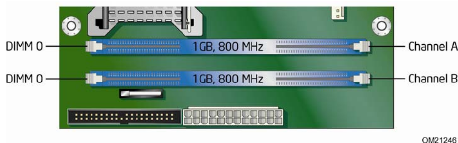
Figure 13. Dual Channel Memory Configuration Example
