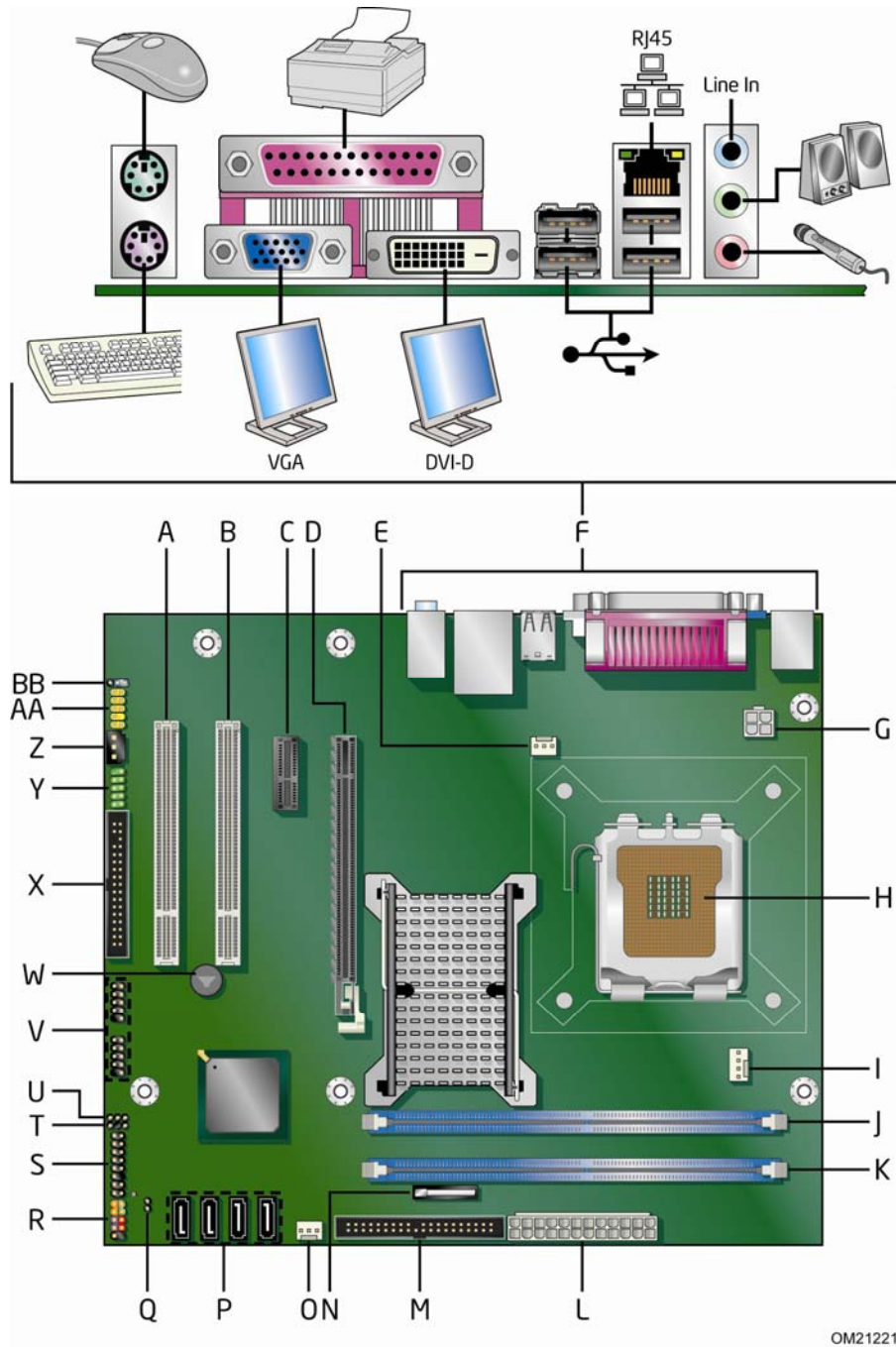
Figure 1. Intel Desktop Board DG41TY Components
