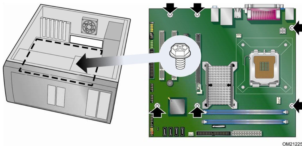
Figure 5. Intel Desktop Board DG41TY Mounting Screw Hole Locations
