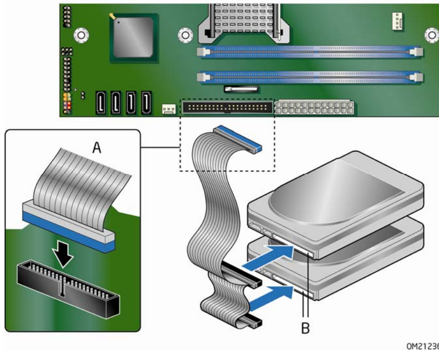
Figure 19. Connecting the IDE Cable
