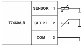
Fig. 9. Circuitry of T7460A,B Wall Modules
